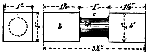
FIG. 60.—TEST-PIECE.
